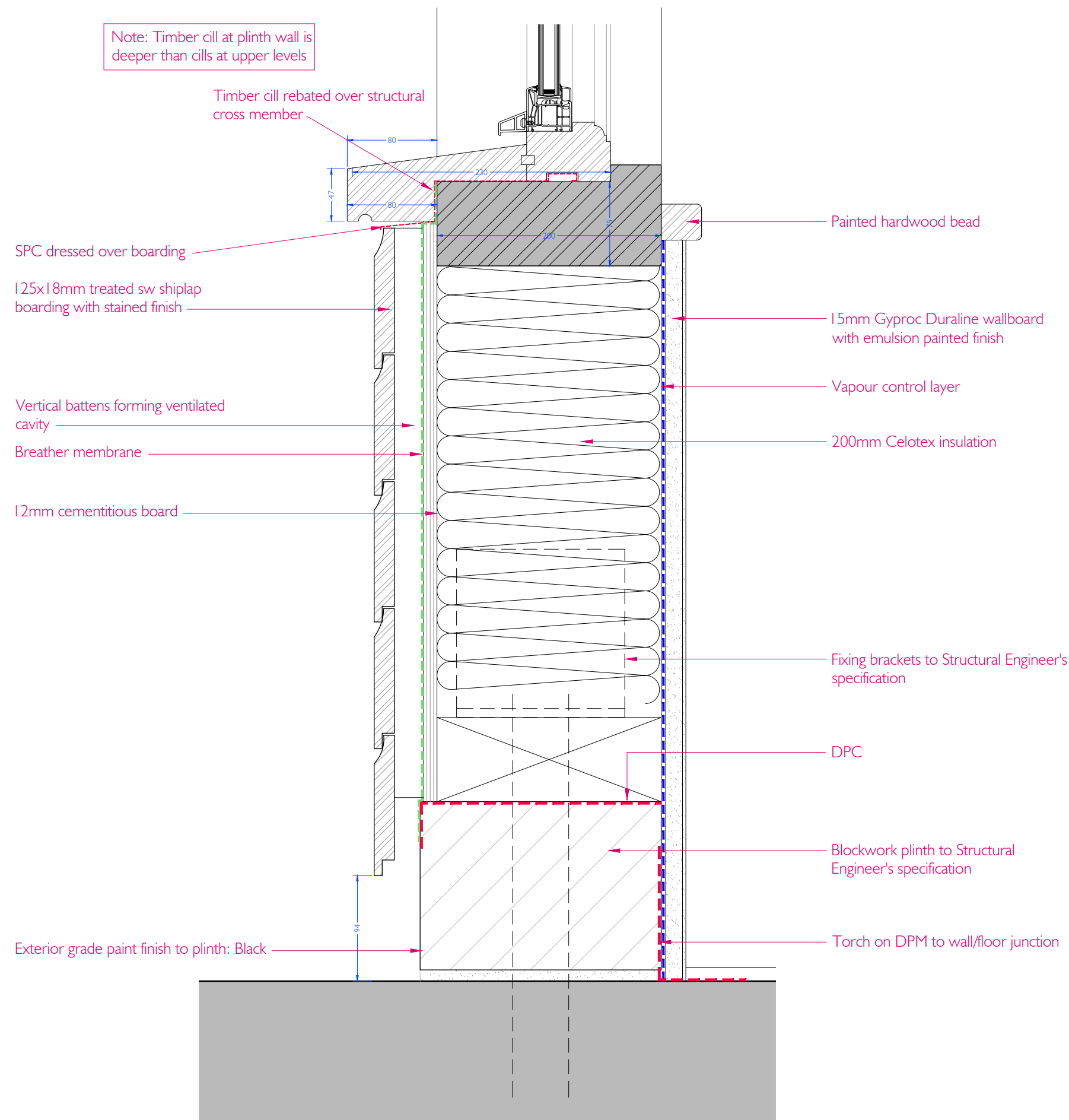
A - TIMBER FRAMED FLANK WALL SECTION DETAIL
